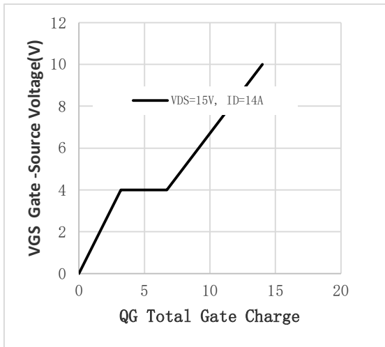
Fig.1 Gate-Charge Characteristics
