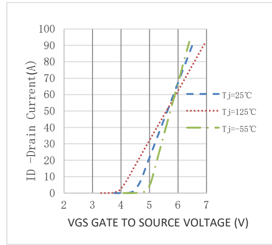
Figure 10. Transfer Characteristics
