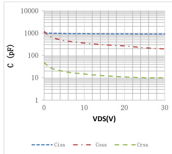
Fig.2 Capacitance Characteristics
