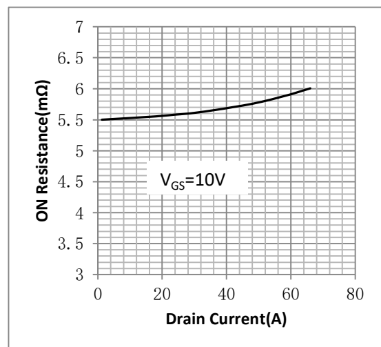
Fig.6 Resistance V.S Drain Current
