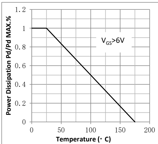
Fig.3 Power Dissipation
